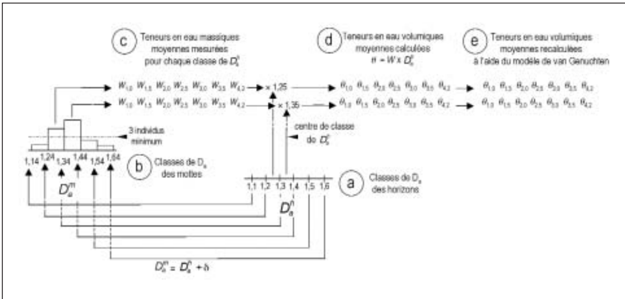
Figure 3 - Detailed presentation of the approach that uses the horizon and clod bulk density to establish class pedotransfer functions.
