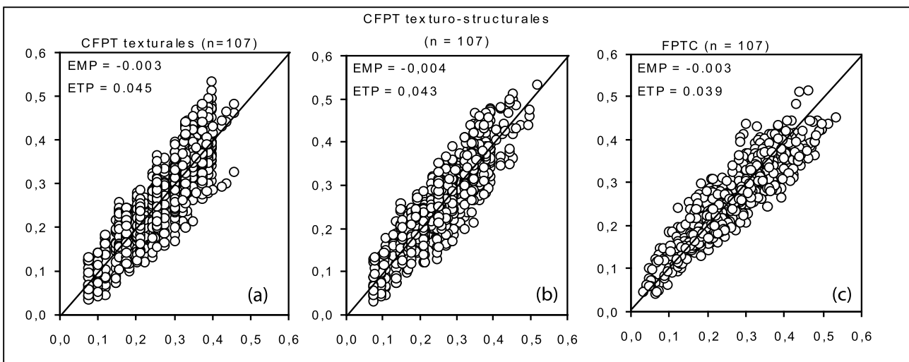
Figure 2 - Validity of the textural class-PTFs (a), texturo-structural PTFs (b) and continuous-PTFs (c) developed with SOLHYDRO 1.0.
