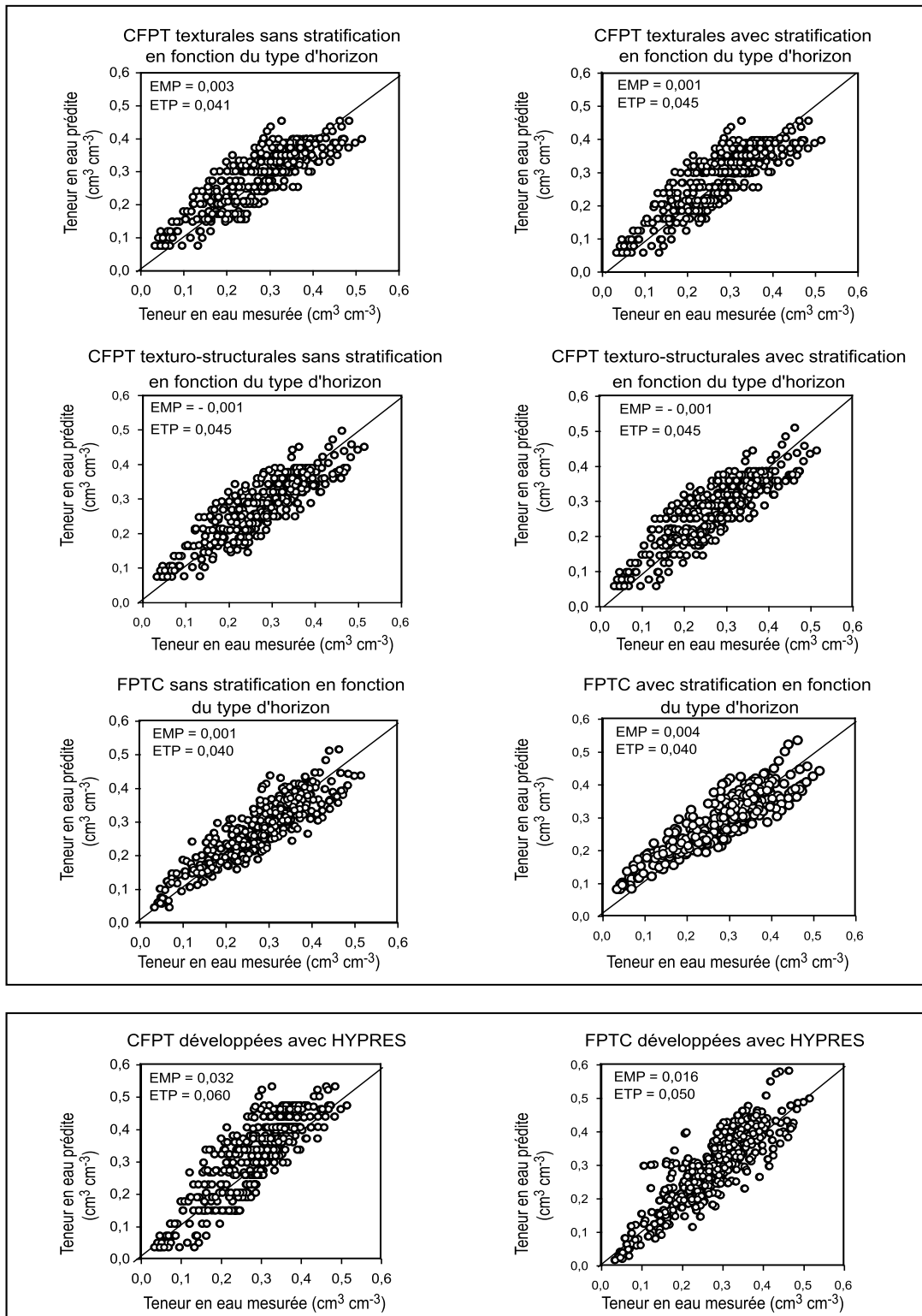
Figure 4 - Validity of the class- and continuous-PTFs developed with SOLHYDRO 1.0 and HYPRES for subsoils (n = 68).
