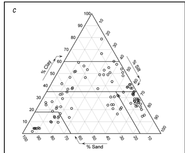
Figure 1 - Triangle of texture used (CEC, 1985) (a), texture of the horizons used to establish the class pedotransfer functions (PTFs) (b) and of those used to test their validity (c).
