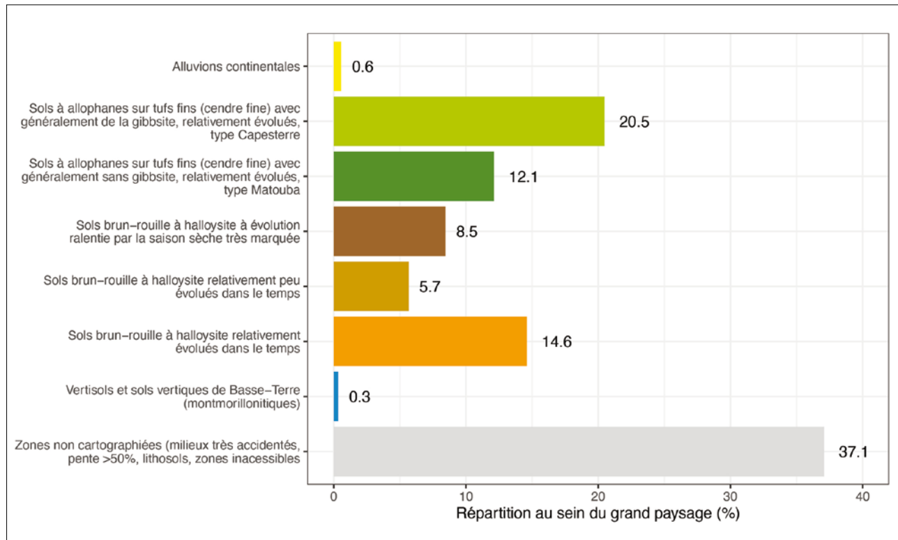
Figure 6: Soils distributions in the landscape GP10.
