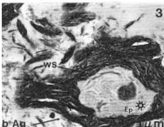
Bacterial aggregate with wavy
