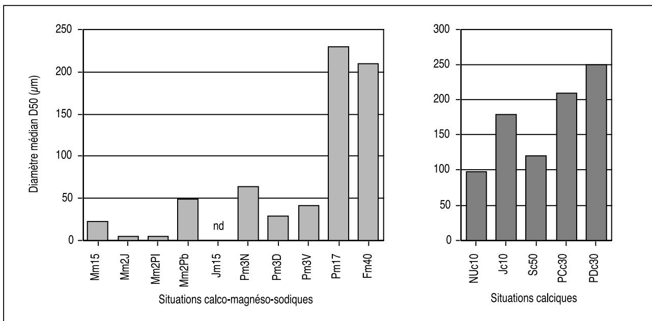
Figure 2 - Mean Diameter D50 ( \mu\text{m} ) of 1-2 mm aggregates after 2 hours shaking in water for different situations.
