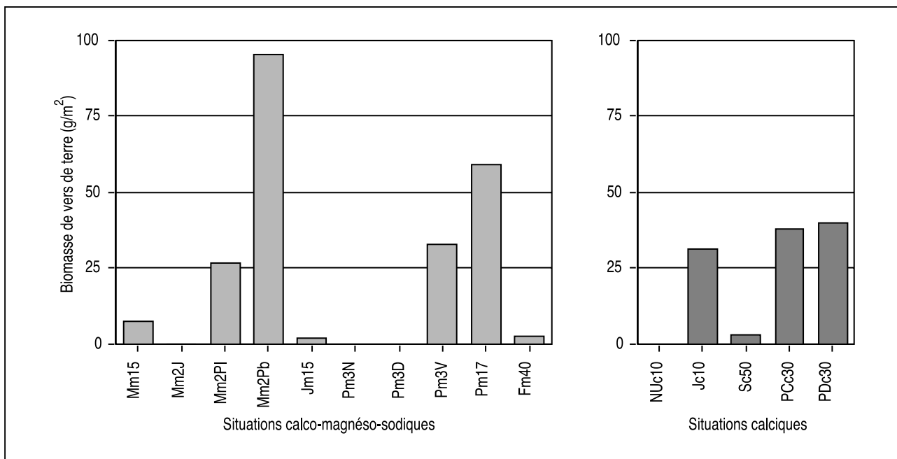
Figure 4 - Earthworm biomasses ( \text{g/m}^2 ) in different situations (0-30 cm depth).
