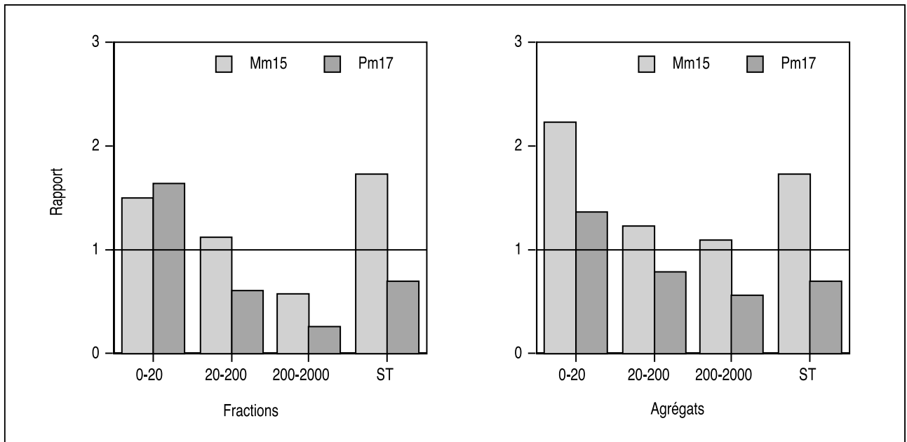
Figure 10 - r ratio measured for Vertisols (0-10 cm depth) under an old pasture Pm17 and an old gardening crop Mm15 (bulk soil ST, size fractions and aggregates).
